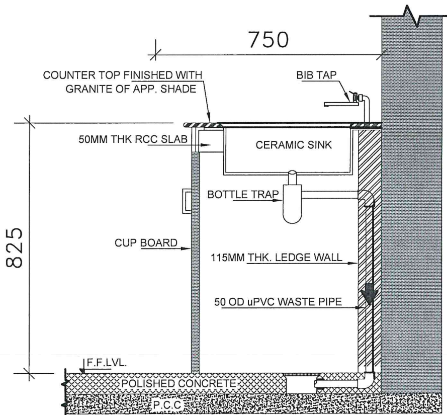
LAB SINK - SECTION
